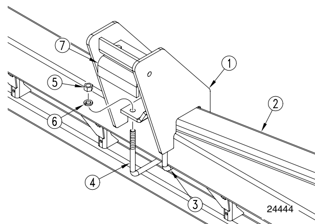
Figure 3 Secure Weight Bracket to Frame
