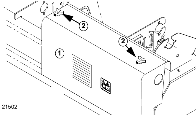
Figure 3-1 Chain Guard
