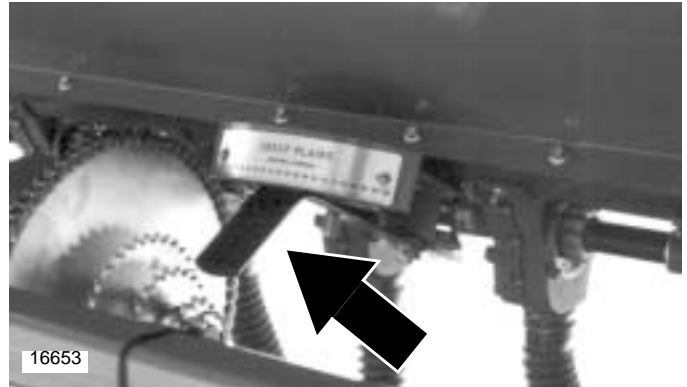
Figure 3-3 Seed-Rate Handle
