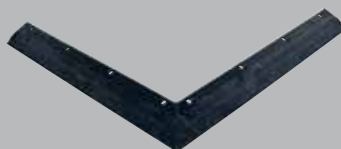
4 1/2" SHALLOW PITCH BLADES - The standard shallow pitch 4 1/2" blades allow shallow tillage and finishing with minimum ridging and lower horsepower requirements. This blade is recommended if higher tillage speeds and shallower tillage depths are desired.
